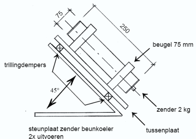
Steun ultrasoon systeem beunkoelers
